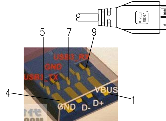
USB 3.0 A M-PIN 3D SPEC.
